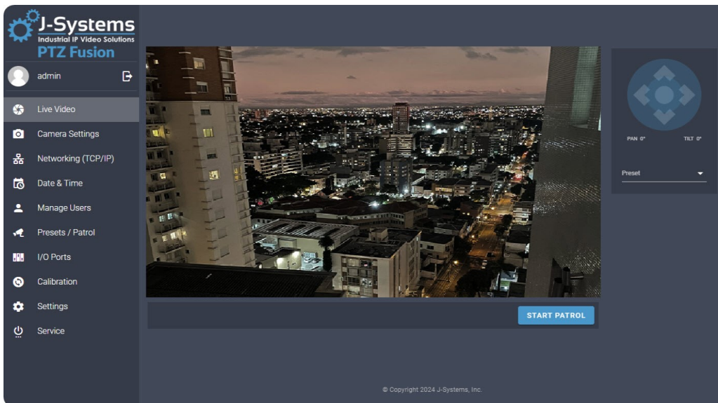
PTZFusion Lite-13 Web Interface with ONVIF Camera
